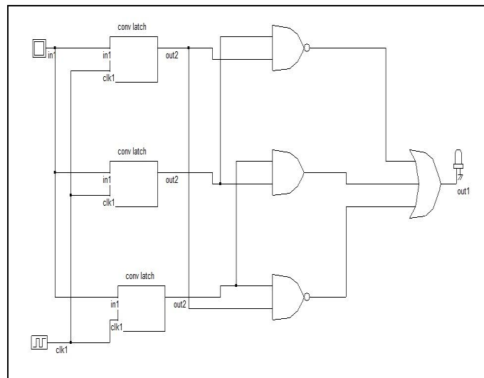
Figure 2: TMR Latch
