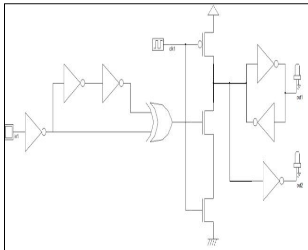
Figure 3: XOR-TD
