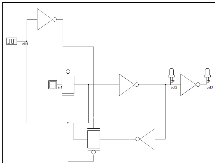
Figure 7: Conventional Latch
