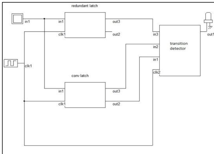
Figure 6: Proposed Latch
