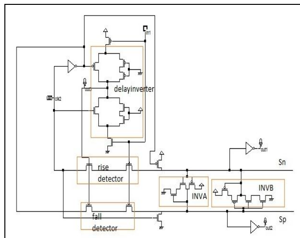
Figure 4: Proposed TD
