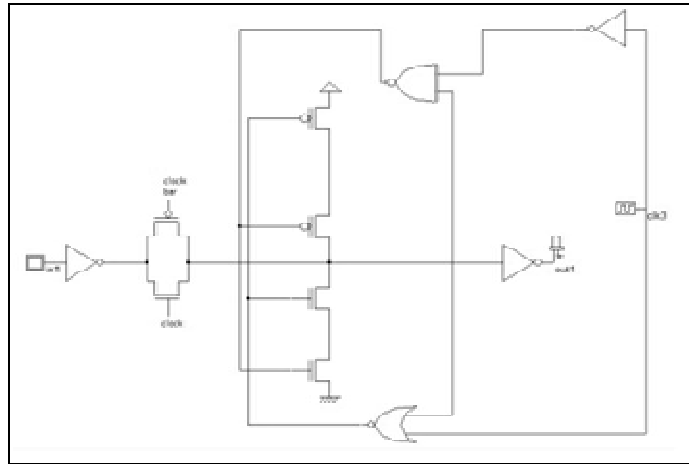
Figure 1: SIN-HR-SUB Latch
