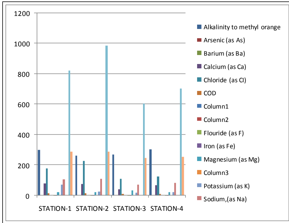
Figure 3: Observed Phycico-Chemical Parameters of Stations-1,2,3 & 4 X-Parameter Y-Units in mg/l
