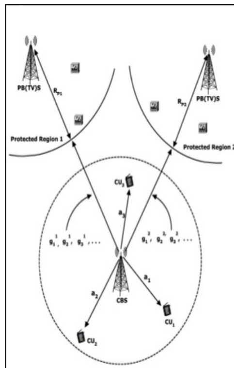
Figure 1: System architecture
