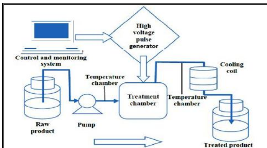
Figure 1: Flow chart of a PEF food processing system with basic component (Maged et al. , 2012)
