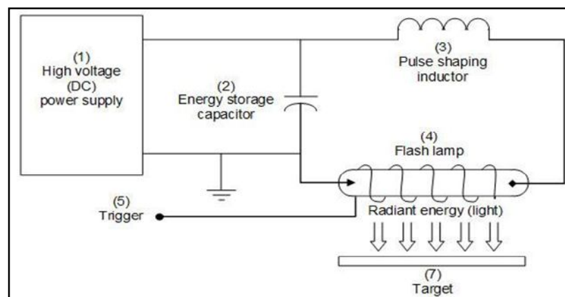
Figure 3: Functional diagram of a high-intensity pulsed-light system. (Adapted from Xenon Corp., 2005)
