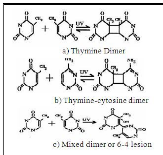
Figure 2: Formation of Thymine Dimer, Thymine-cytosine dimer and mixed dimer (Setlow et al. , 1966).
