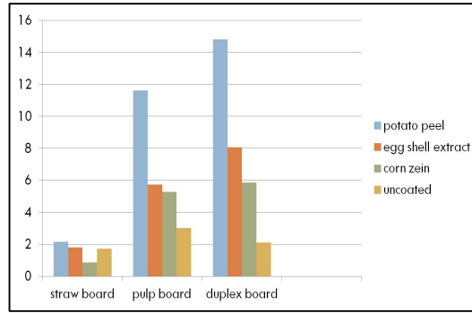
Figure 1: Graphical Representation Of Tensile Strength
