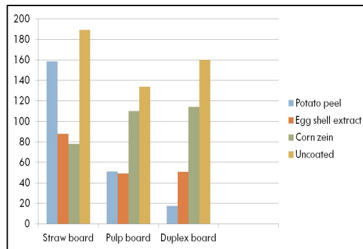
Figure 2: Graphical Representation of Water Absorption Results
