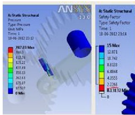
Figure 8: Result for Teeth 32
