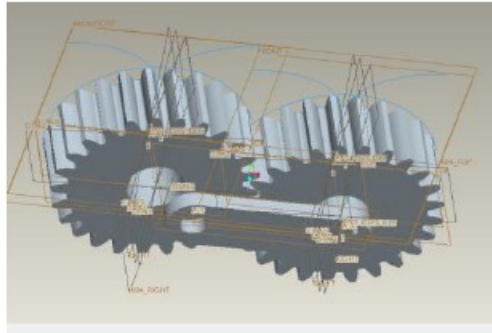
Figure 5: Assembly of Parametric Spur Gear Model
