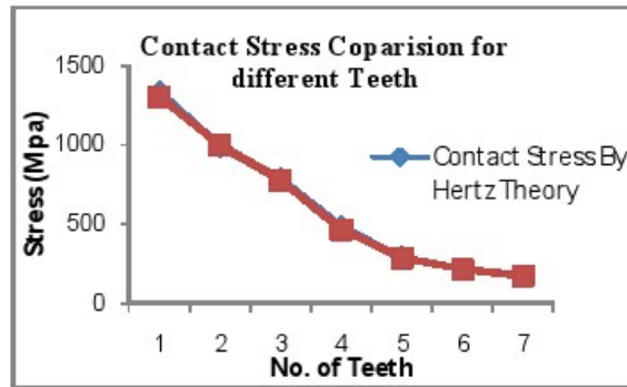
Graph 3: Graphical representation for contact stresses comparison for different Teeth
