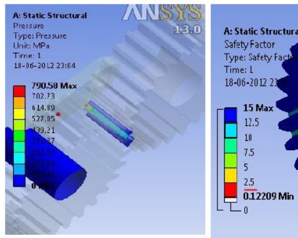
Figure 6: .FEM Result for Teeth 24
