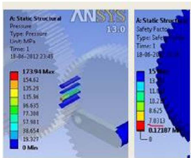
Figure 12: Result for Teeth 68
