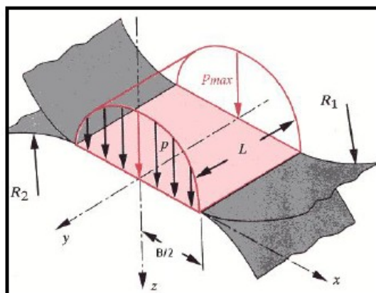
Fig 3: Ellipsoidal-prism pressure distribution
