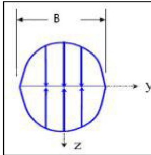
Figure 2: Elliptical stress distribution across the width
