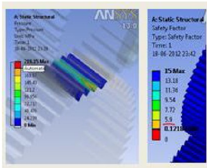
Figure 11: Result for Teeth 64
