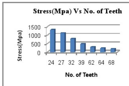
Graph 1: Graph for Hertzian analytical results for different Teeth
