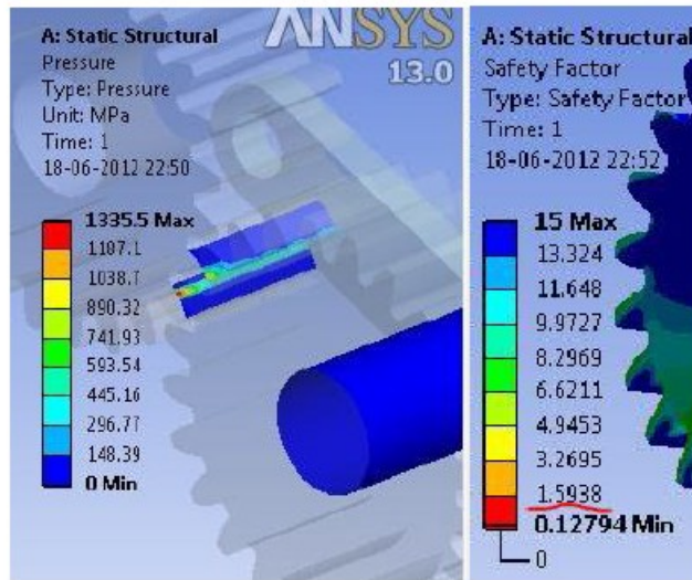
Figure 6: .FEM Result for Teeth 24
