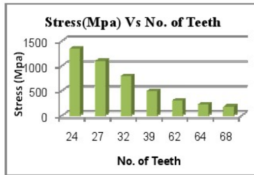
Graph 2: Graph for ANSYS FEM results for different Teeth
