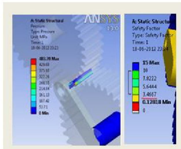
Figure 9: Result for Teeth 39
