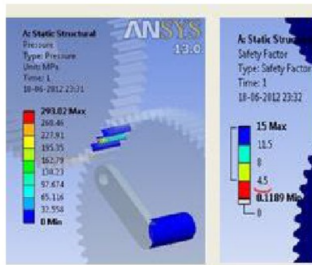
Figure 10: Result for Teeth 62
