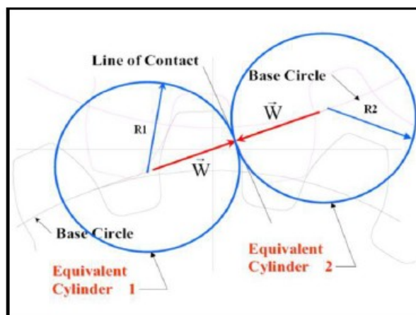
Figure 4: Equivalent contacting cylinder
