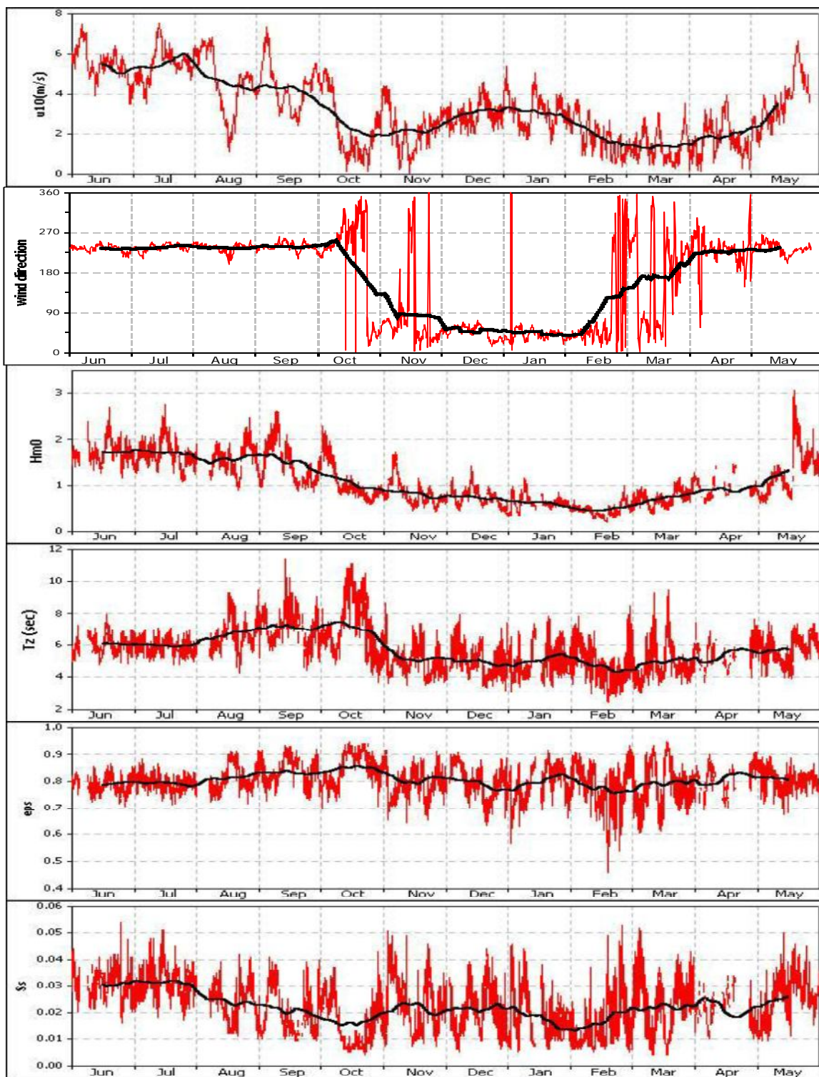
Figure 2: Seasonal variation of wind speed (U10), wind direction (angle of wind vector in degrees w.r.t north), significant wave height (Hs), zero upcross period (Tz), spectral band width parameter ( \epsilon ) and significant steepness (Ss). Thin line shows the measured data with 30min interval and thick line shows 30 days moving average.
