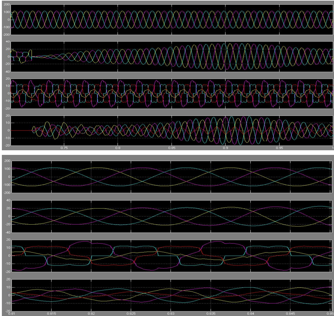
Figure 5: Simulation results: (a) Grid voltages, (b) Grid Currents (c) Unbalanced load currents, (d) Inverter Currents
