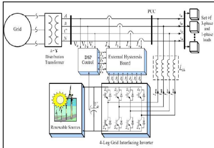
Figure 1: Schematic of proposed renewable based distributed generation system
