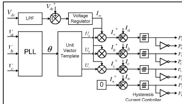
Figure 3: Block diagram representation of grid-interfacing inverter control
