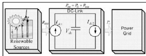
Figure 2: DC-Link equivalent diagram.
