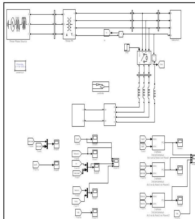
Figure 4: mat lab simulation design
