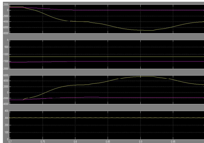
Figure 6: Simulation results: (a) PQ-Grid, (b) PQ-Load, (c) PQ-Inverter, (d) dc-link voltage.
