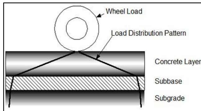
Figure 2: Load distribution of rigid pavement
