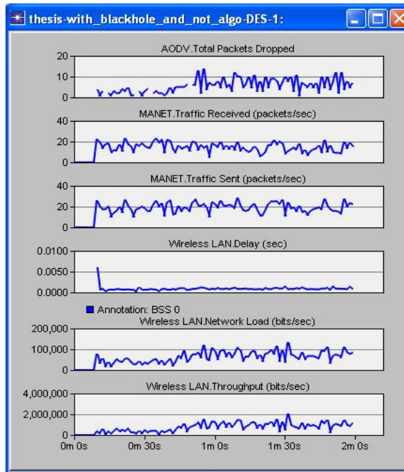
Figure 7: Second Scenario results with black hole but no prevention algorithm
