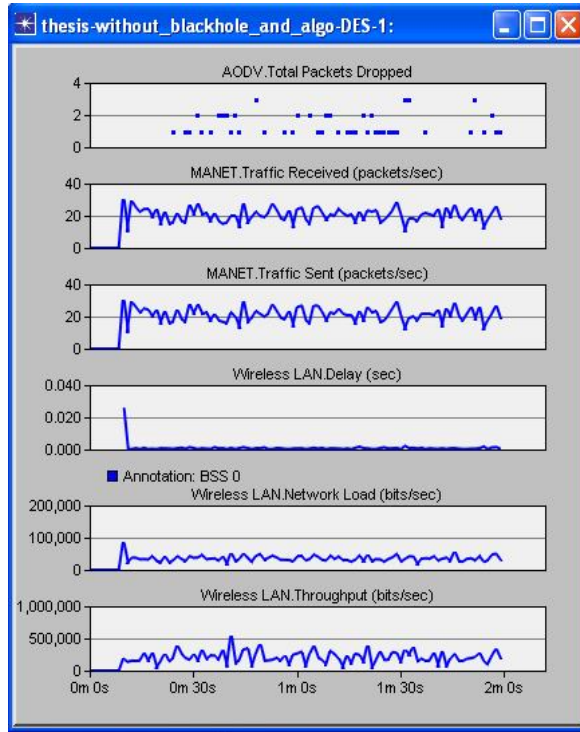
Figure 6: First Scenario results without black hole and proposed algorithm
