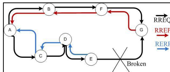
Figure 2: Route Error Message in AODV
