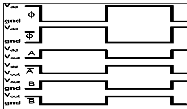
Figure 3: detailed view of signals at internal points of dual sc converter
