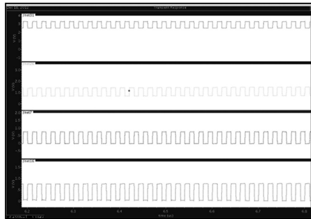
Figure 6: timing diagram of cross-coupled dual sc converter
