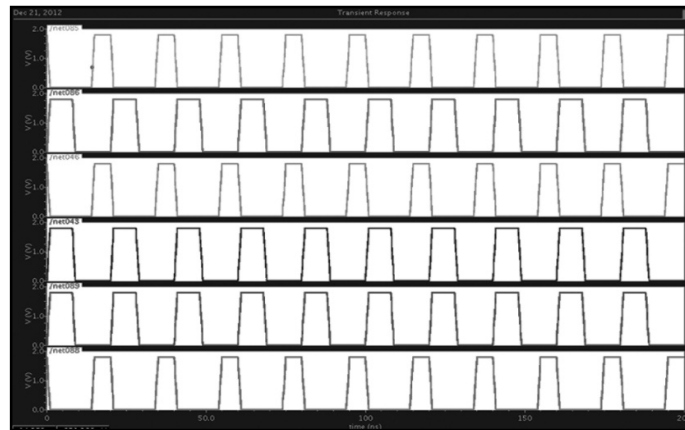
Figure 8: timing diagram of NRTI converter
