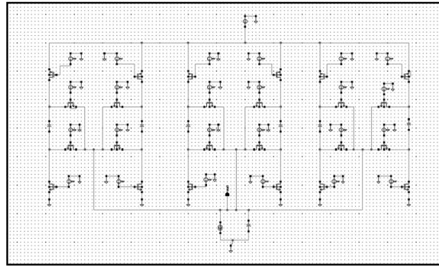
Figure 7: diagram of 3-element cross-coupled NRTI converter
