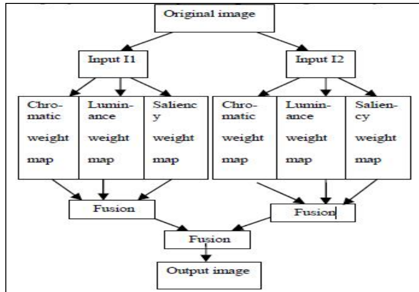
Figure 2: The Outline Of Our Algorithm
