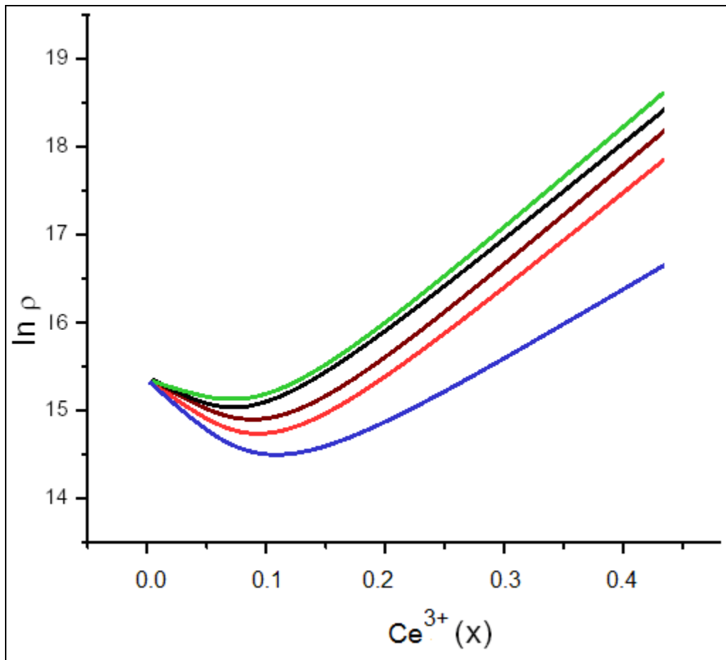
Figure 1: Variation of resistivity with concentration
