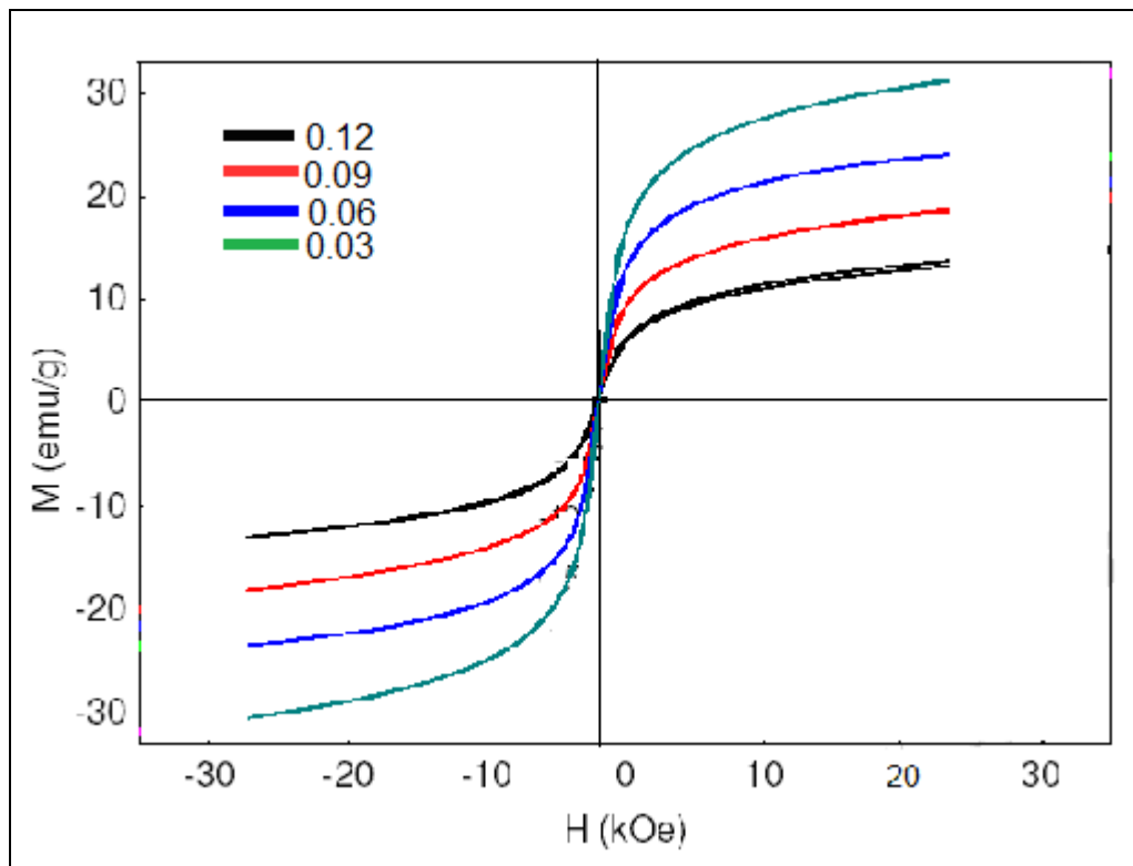
Figure 2: Hysteresis loop of NiCe_xFe_{2-x}O_4 at different x ( x=0.00, 0.03, 0.06, 0.09, 0.12 )
