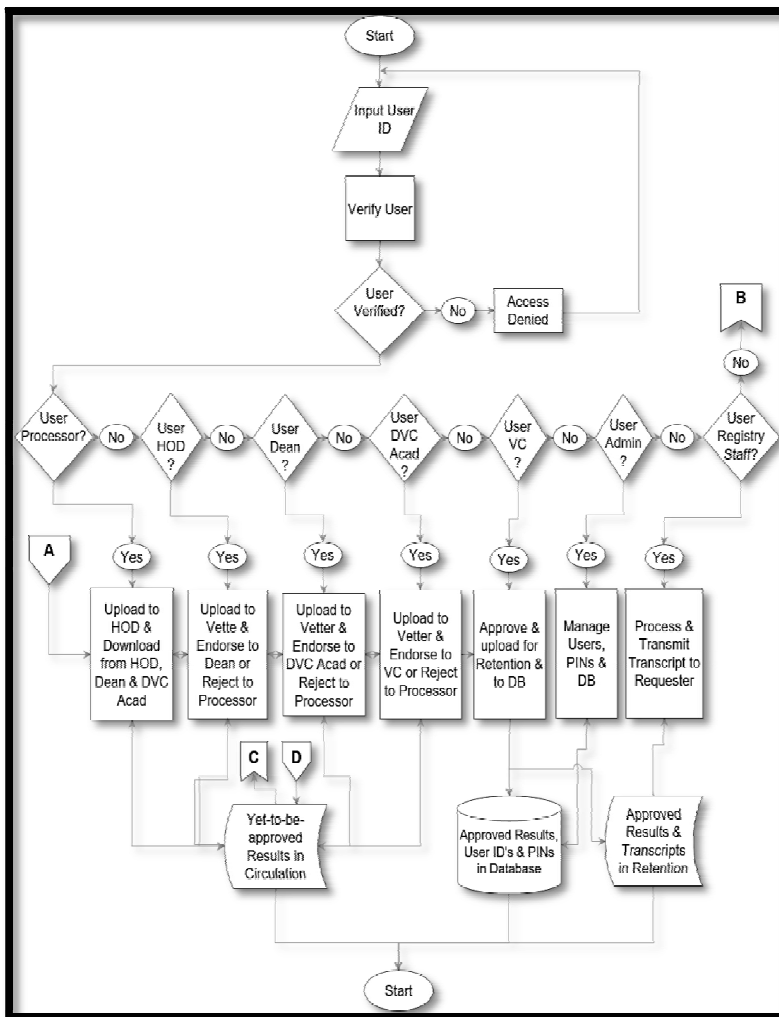
Figure 13(A): HRPMS Results Management Processing Model Flowchart Keys: A = Incoming Files Link from Export Folder on Result Processor System, B = Link to Other Users, C & D = Outgoing and Incoming Transit Files Links from and to Circulation Folder on the Server
