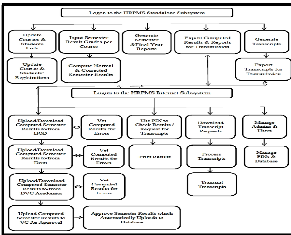
Figure 11: HRPMS High Level Model Diagram
