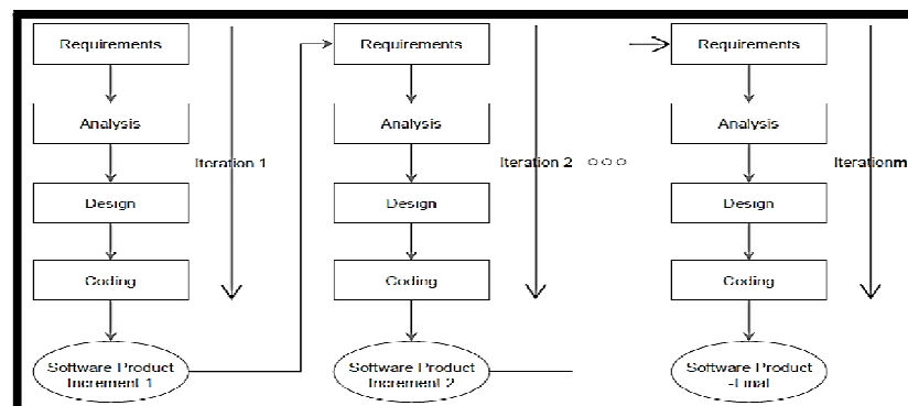
Figure 5: Scrum Agile Software Development Model (Michaels, 2013)
