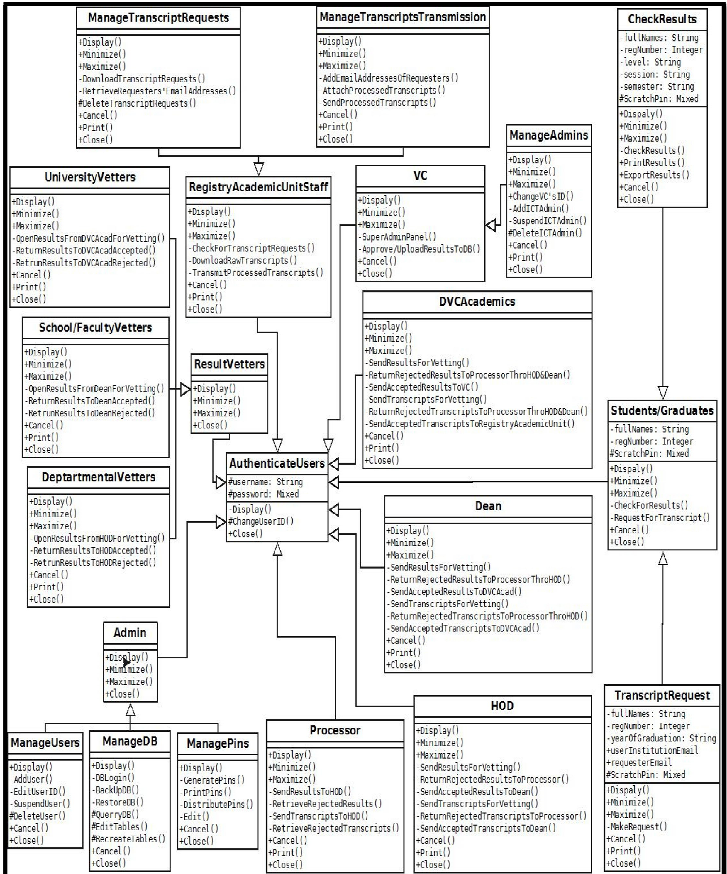
Figure 18: Class Model Diagram of HRMS Client-Server Subsystem
