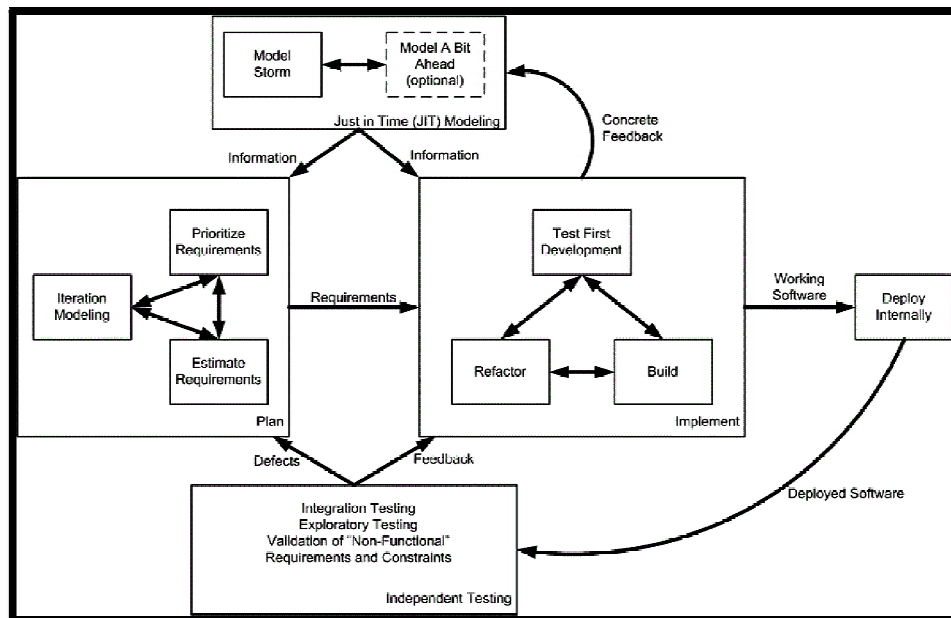
Figure 2: Agile Development Process (Theunissen, Boake, & Kourie, 2005)
