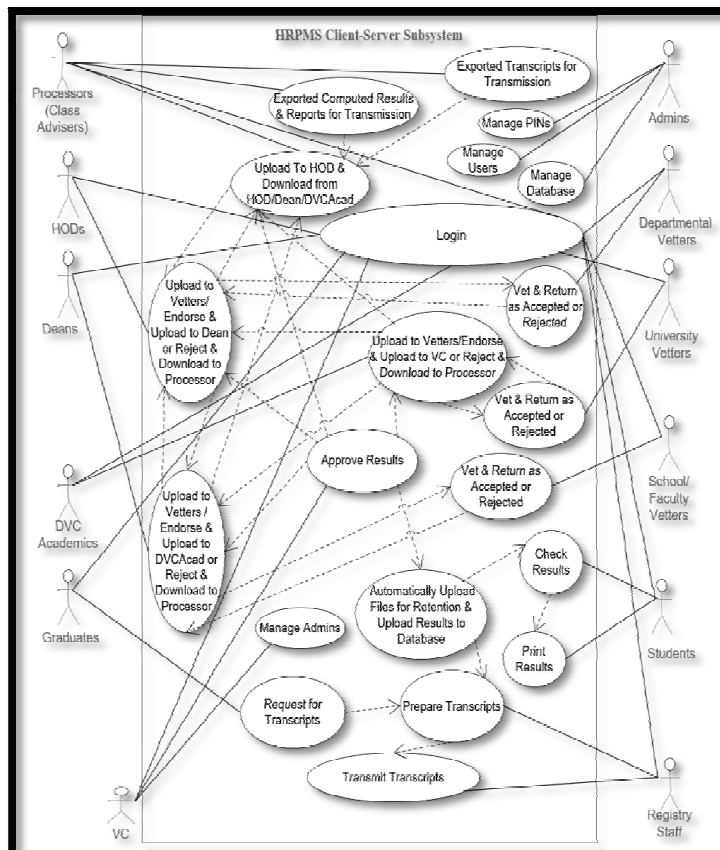
Figure 16: HRPMS Client-Server Subsystem Use Case Model Diagram
