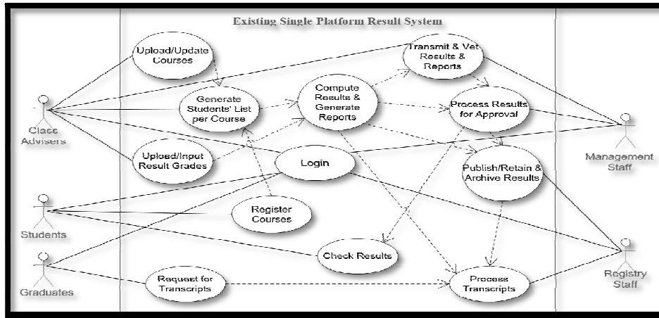
Figure 9: Use Case Diagram of the Single-Platform Existing System
