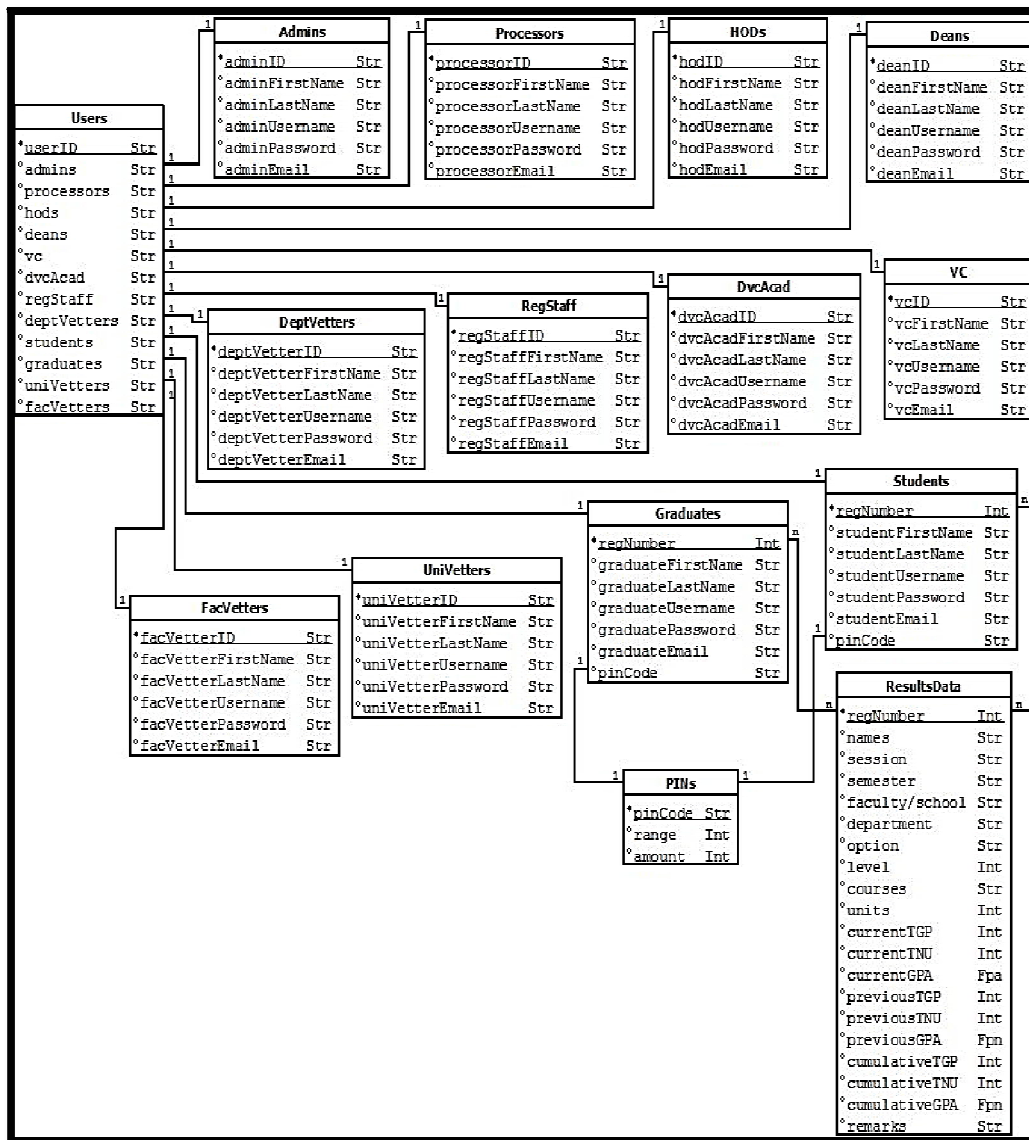
Figure 19: HRPMS Database Entity-Relationship Model Diagram
