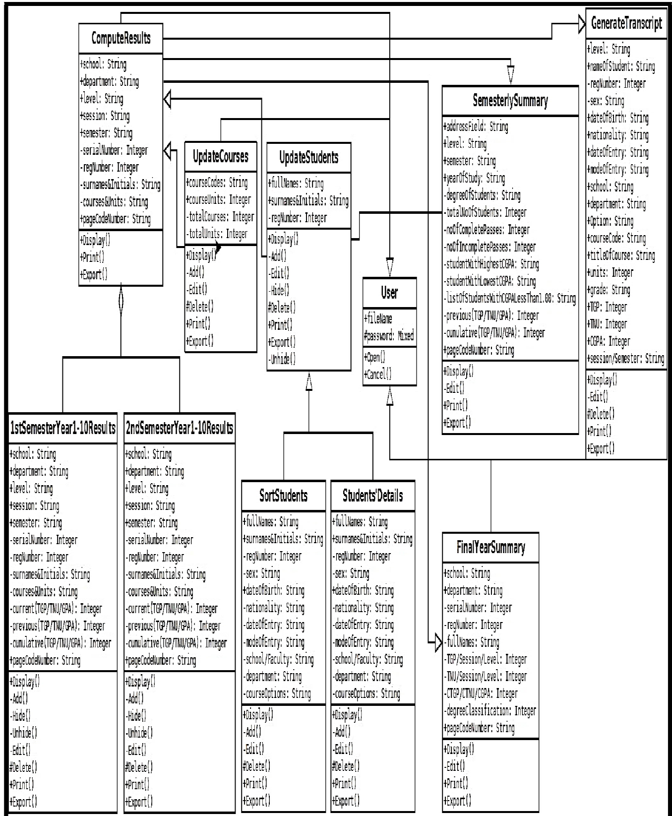
Figure 17: Class Model Diagram of HRPMS Standalone Subsystem
