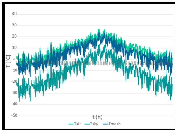
Figure 3: Comparison of Temperatures
