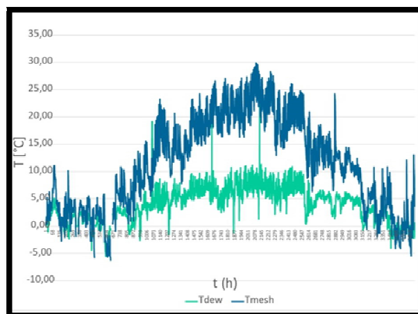
Figure 4: Dew Formation
